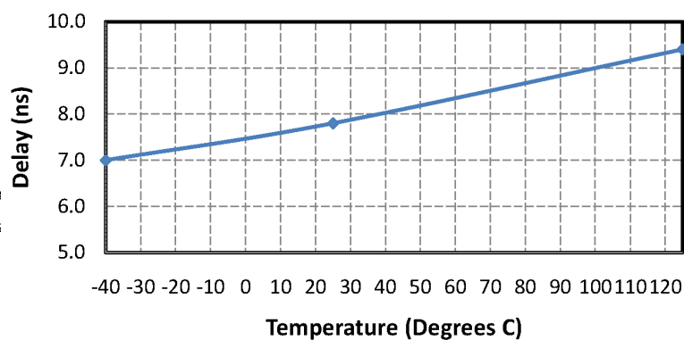
Figure 3.9. Propagation Delay vs. Temperature
