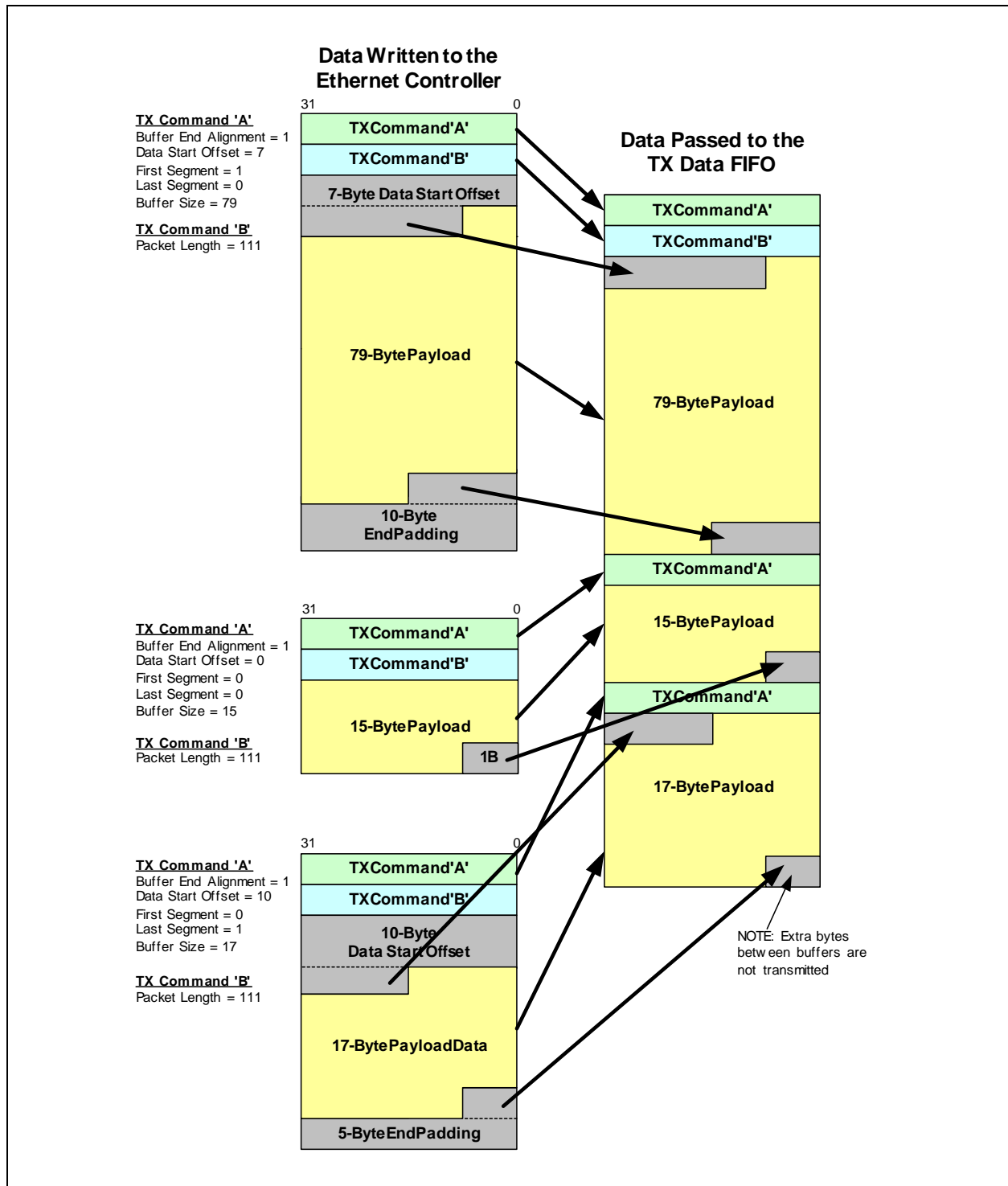
FIGURE 3-21: TX EXAMPLE 1
