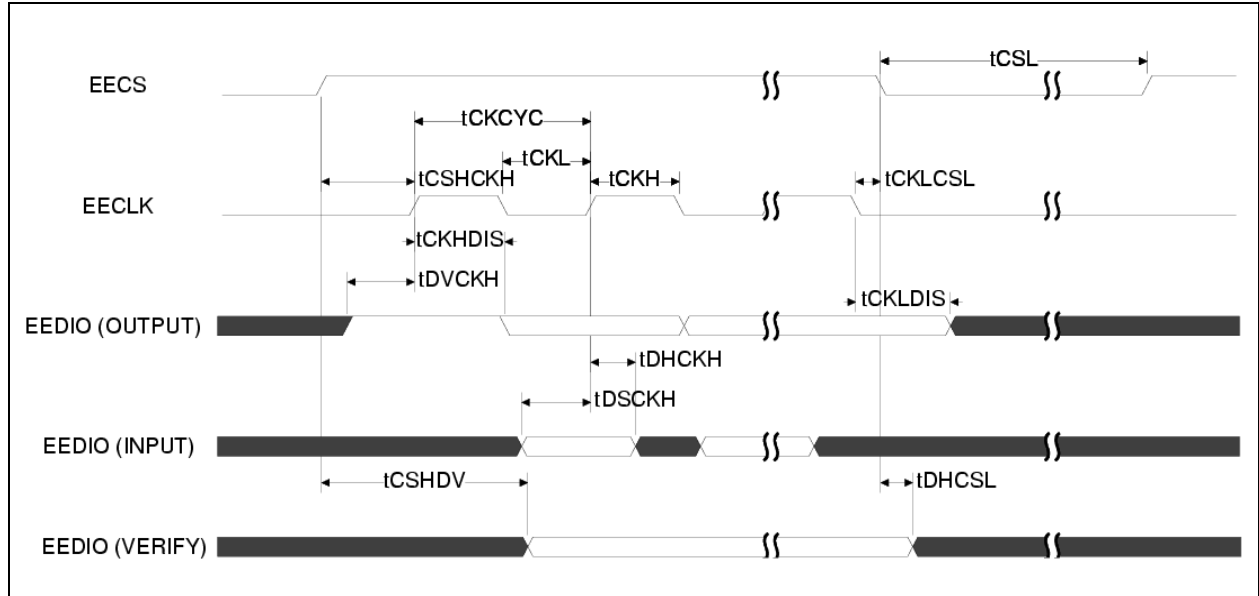
FIGURE 6-8: EEPROM TIMING
