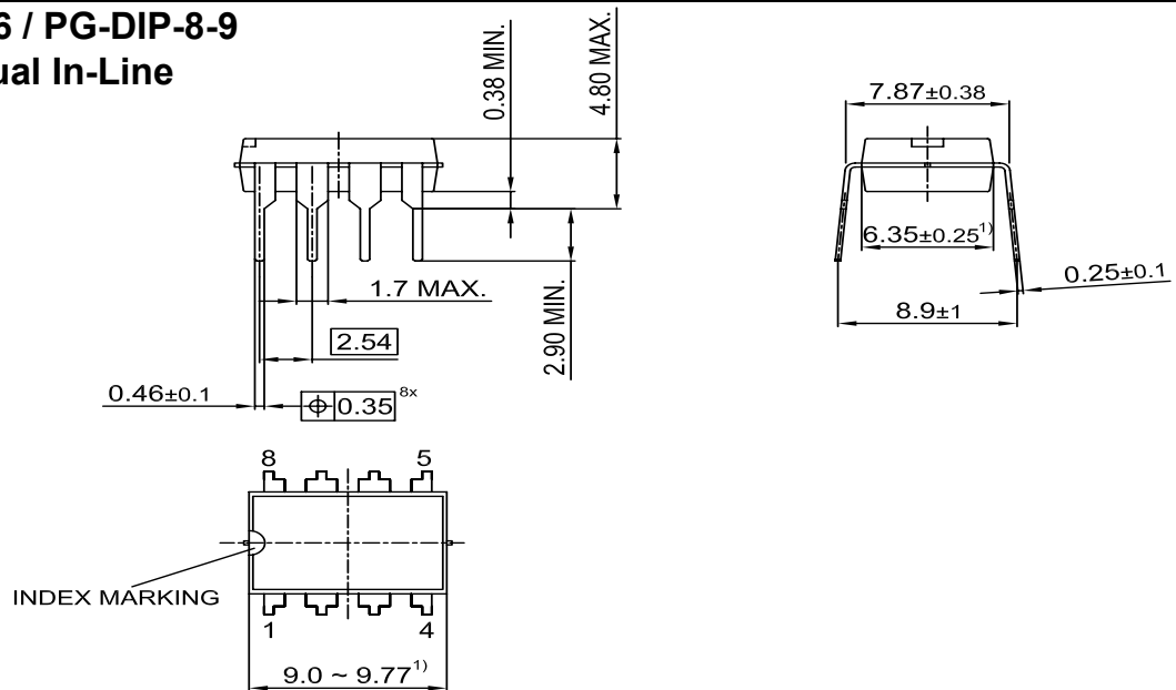
Figure 33 PG-DIP-8 (Pb-free lead plating Plastic Dual-in-Line Outline)
