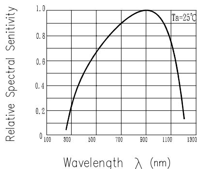
Fig.5 Spectral Sensitivity
