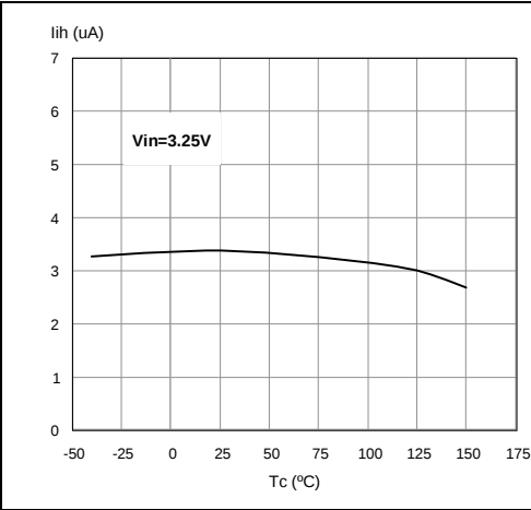
Figure 10. Status leakage current
