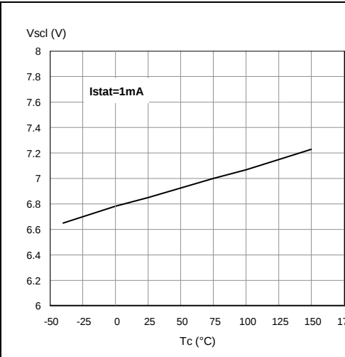
Figure 12. Status clamp voltage
