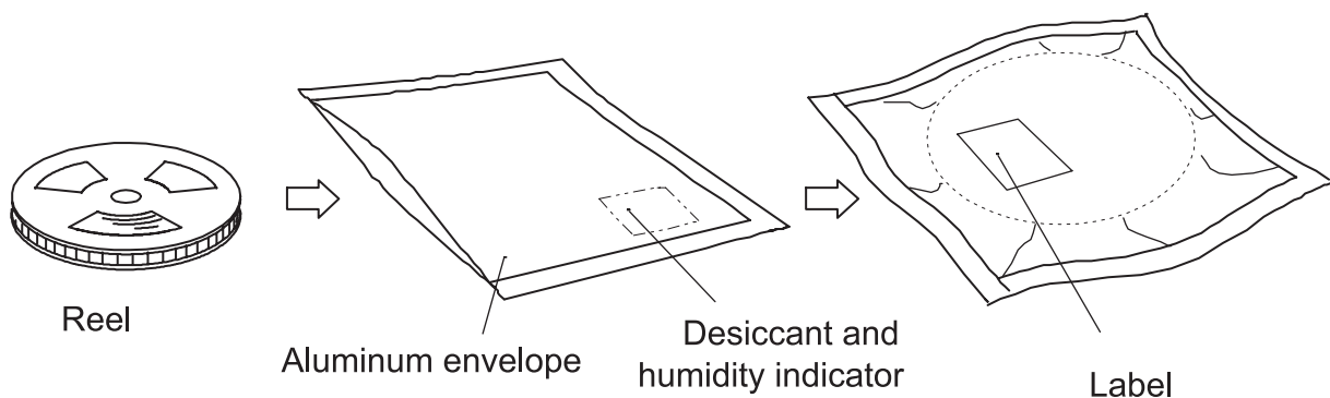
Figure 7. ZHX1403 Packaging
