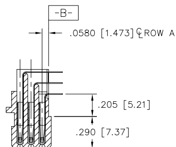
SECTION X-X
