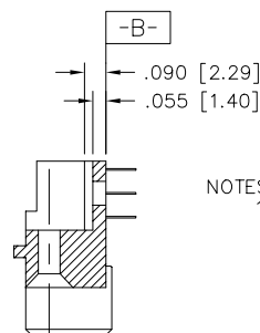
SECTION W-W
