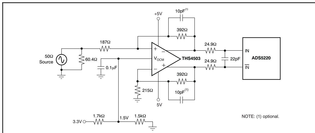
Figure 23. Using the THS4503 Differential Amplifier (Gain = 2) to Drive the ADS5220 in a DC-Coupled Configuration
