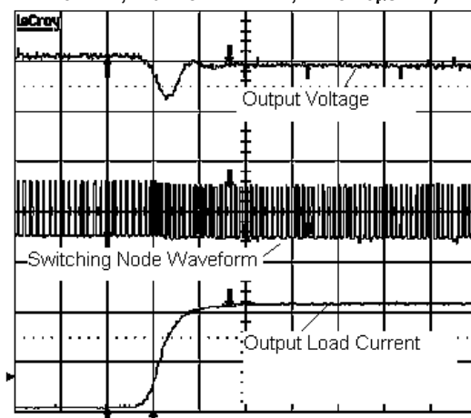
Load Transient Test ( V_{IN}=5V , V_{OUT}=1.2V , I_{OUT}=0A to 4A , Forced Continuous Conduction Mode, L_{OUT}=1.3\mu H , C_{OUT}=3 \times 22\mu F , Channel 1: 50mV/Div, Channel 2: 5V/Div, Channel 4: 2A/Div, Time: 10 \mu s /Div)
