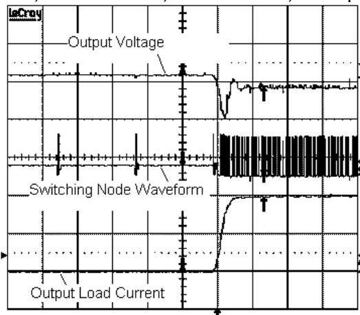
Load Transient Test ( V_{IN}=5V , V_{OUT}=1.2V , I_{OUT}=0A to 4A , PSAVE Mode Enabled, L_{OUT}=1.3\mu H , C_{OUT}=3 \times 22\mu F , Channel 1: 50mV/Div, Channel 2: 5V/Div, Channel 4: 2A/Div, Time: 20μs/Div)
