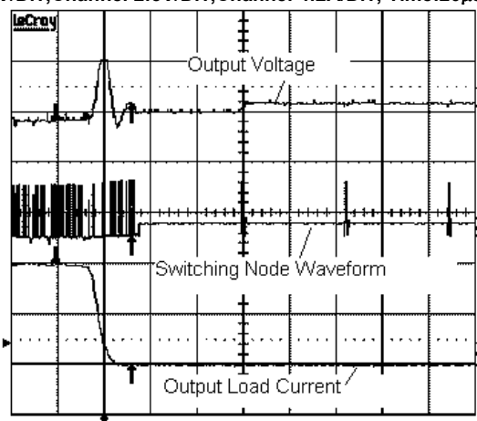
Load Transient Test ( V_{IN}=5V , V_{OUT}=1.2V , I_{OUT}=4A to 0A , PSAVE Mode Enabled, L_{OUT}=1.3\mu H , C_{OUT}=3 \times 22\mu F , Channel 1: 50mV/Div, Channel 2: 5V/Div, Channel 4: 2A/Div, Time: 20μs/Div)
