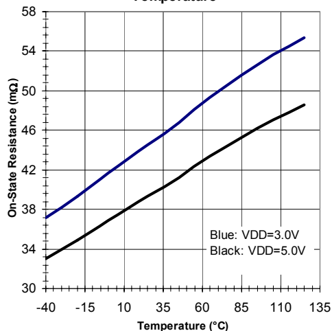
Low Side Switch On-State Resistance vs Temperature
