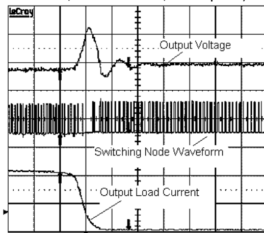
Load Transient Test ( V_{IN}=5V , V_{OUT}=1.2V , I_{OUT}=4A to 0A , Forced Continuous Conduction Mode, L_{OUT}=1.3\mu H , C_{OUT}=3 \times 22\mu F , Channel 1: 50mV/Div, Channel 2: 5V/Div, Channel 4: 2A/Div, Time: 10 \mu s /Div)
