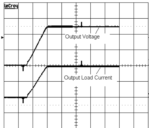
Load Transient Test ( V_{IN}=5V , V_{OUT}=1.2V , I_{OUT}=0A to 4A , Forced Continuous Conduction Mode, L_{OUT}=1.3\mu H , C_{OUT}=3 \times 22\mu F , Channel 1: 50mV/Div, Channel 2: 5V/Div, Channel 4: 2A/Div, Time: 10 \mu s /Div)
