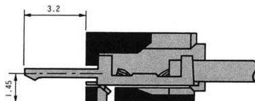
垂直型装着断面 Straight Type Cross Cut Section
