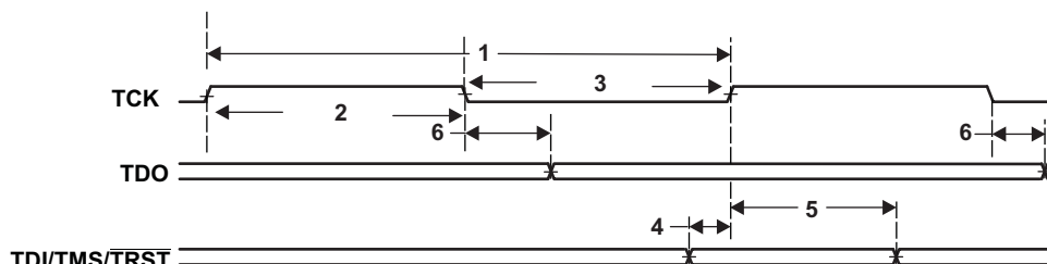
Figure 5-72. JTAG Test-Port Timing
