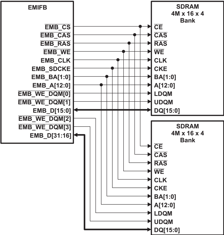
Figure 5-23. EMIFB to Dual 4M × 16 × 4 bank SDRAM Interface
