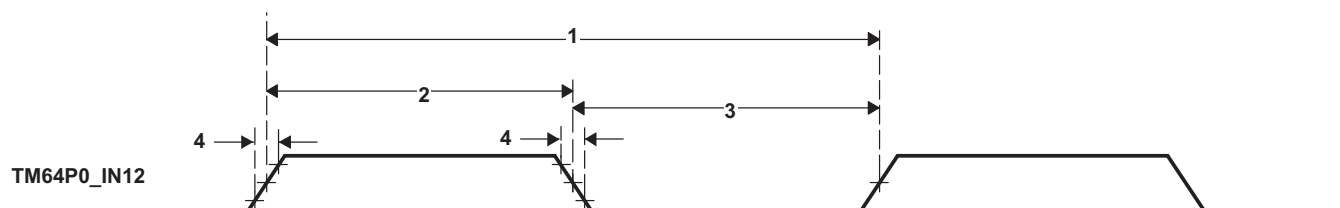
Figure 5-60. Timer Timing
