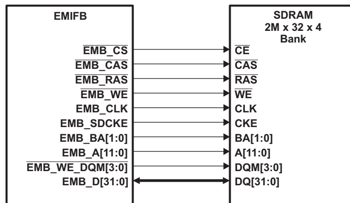
Figure 5-22. EMIFB to 2M × 32 × 4 bank SDRAM Interface
