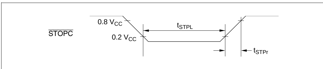
Figure 25-16 \overline{\text{STOPC}} Timing (HD404318 Series)
