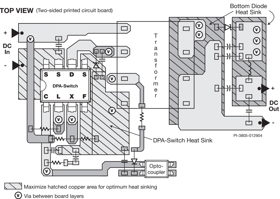
Figure 29. Layout Considerations for DPA-Switch Using G Package.
