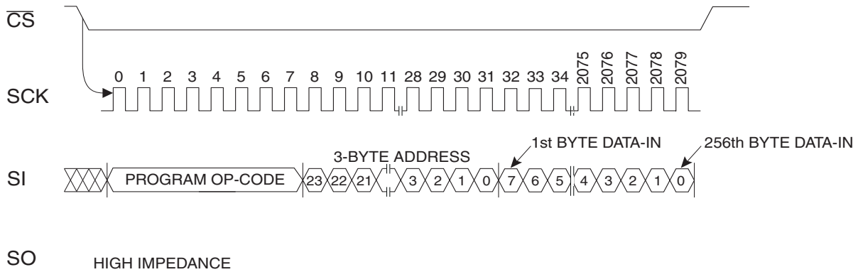
Figure 5-8. PROGRAM Timing
