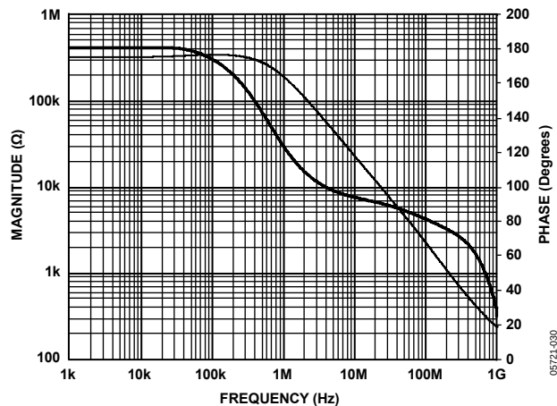
Figure 37. Transimpedance
