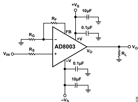
Figure 38. Noninverting Gain
