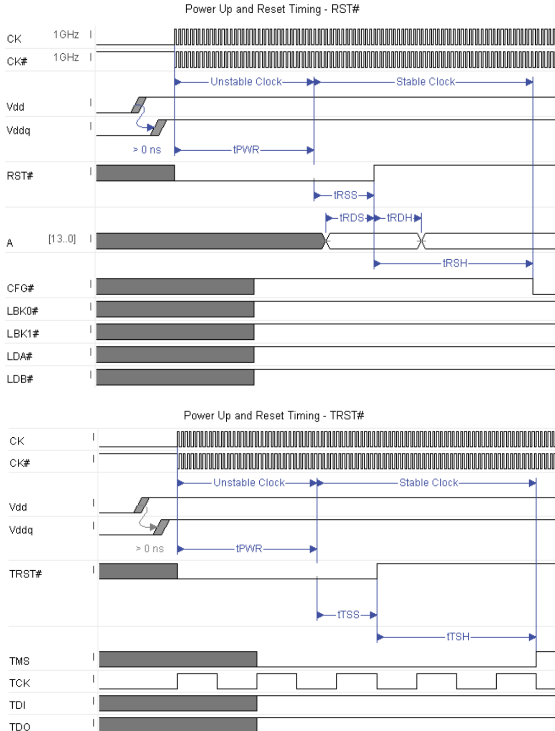
Figure 16. Reset Timings
