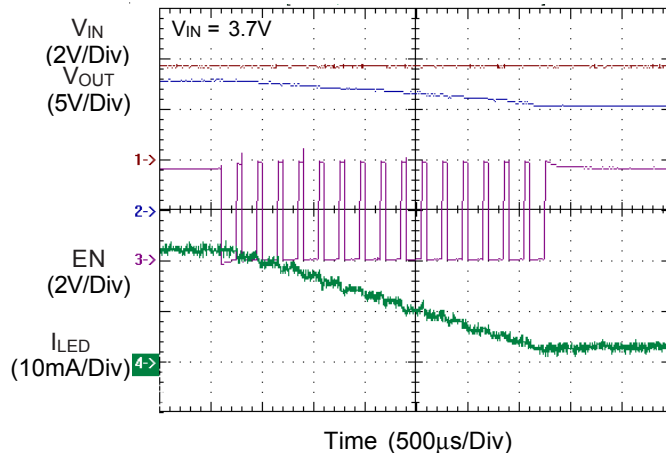
Dimming Operation @ Decrease
