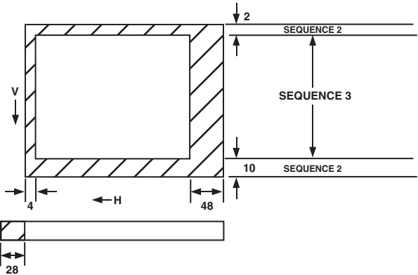
Figure 25. Typical CCD
