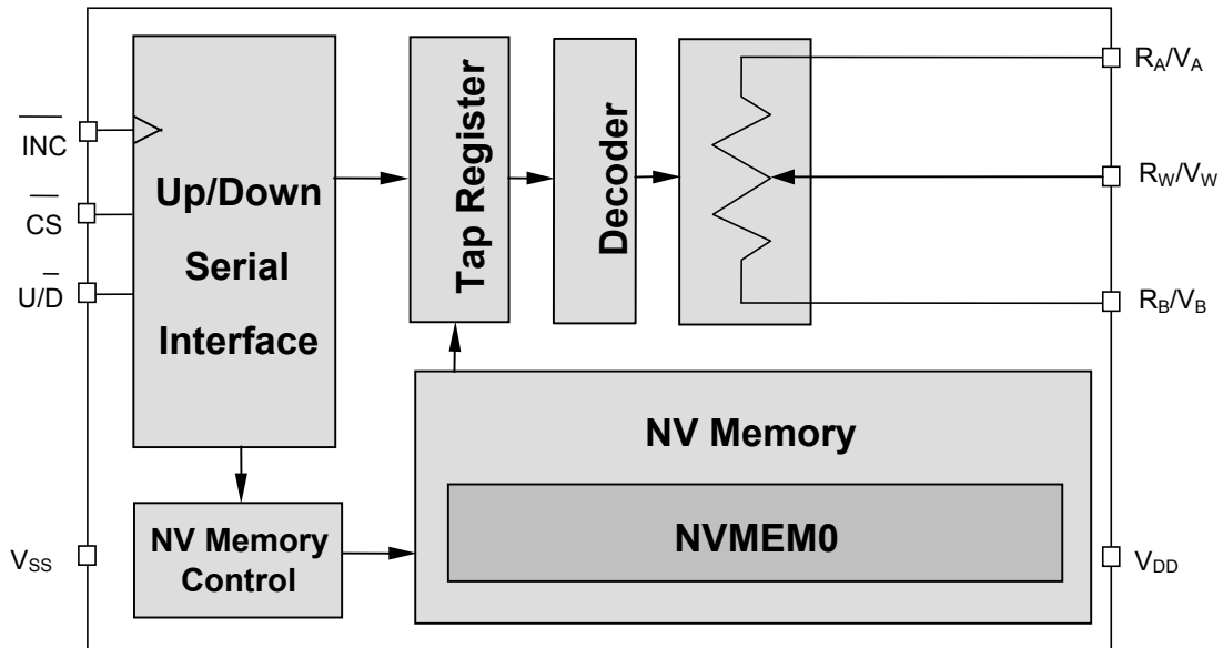
FIGURE 1 – WMS7110 BLOCK DIAGRAM (Rheostat/Divider Mode)
