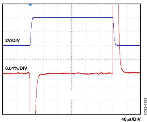
Figure 11. Settling Time
