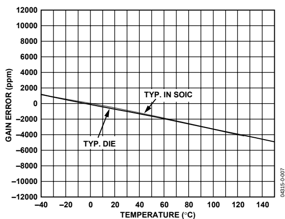
Figure 6. Gain Drift
