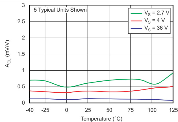
Figure 5-21. Open-Loop Gain vs Temperature
