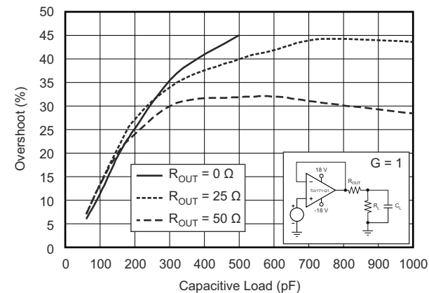
Figure 5-23. Small-Signal Overshoot vs Capacitive Load (100-mV Output Step)
