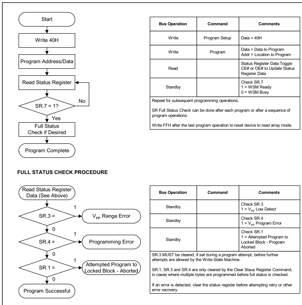
Figure 12. Program Flowchart
