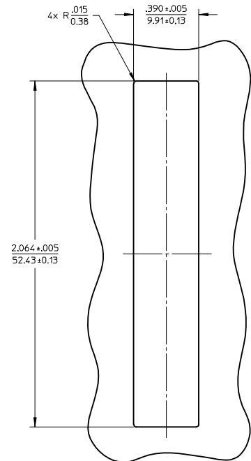
RECOMMENDED MOUNTING PATTERN
