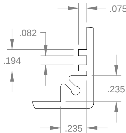
DETAIL C
