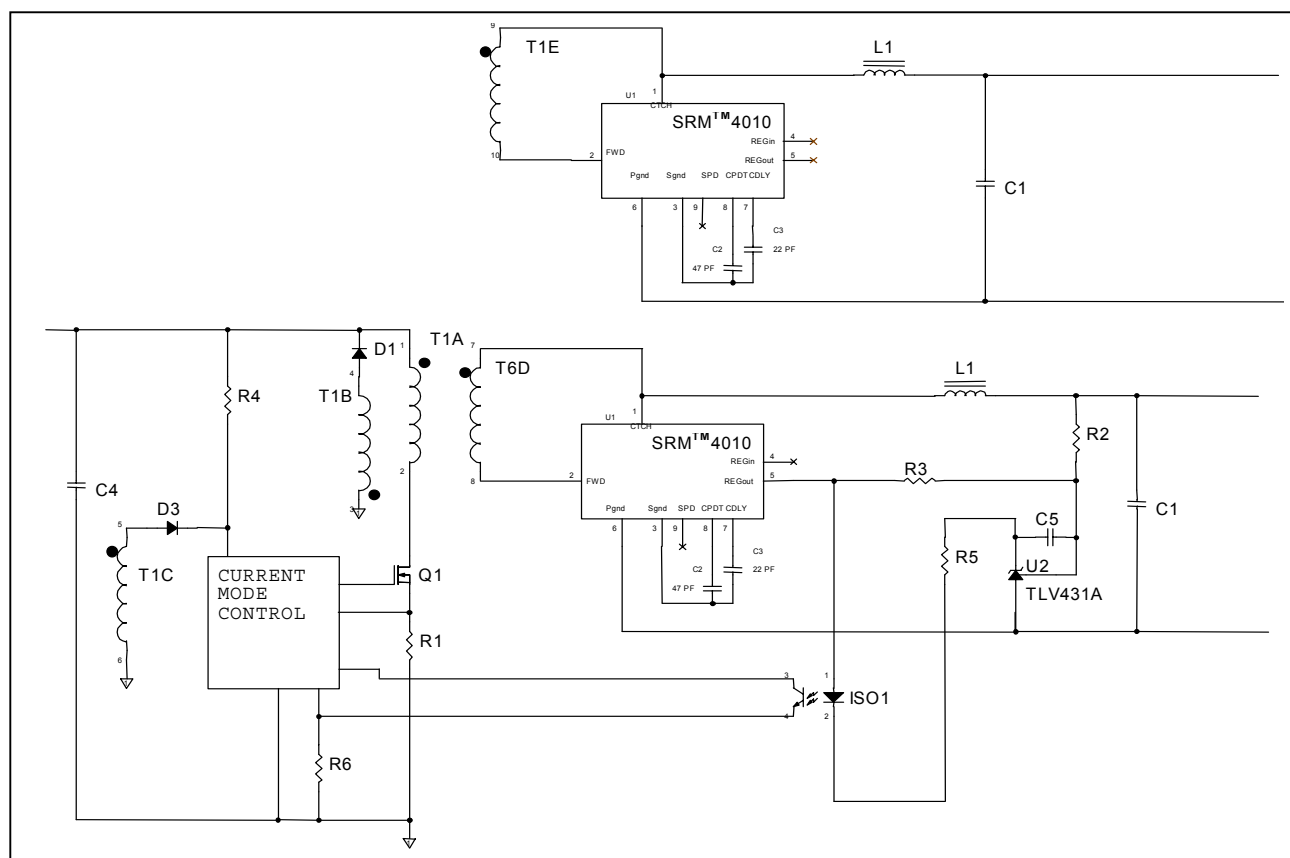
Figure 9 SRM TM 4010 Multiple Output Configuration
