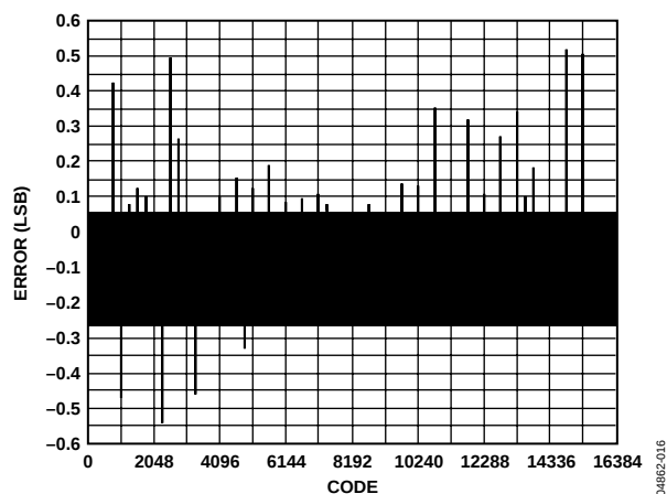
Figure 16. AD9736 DNL, -40°C, 20 mA FS
