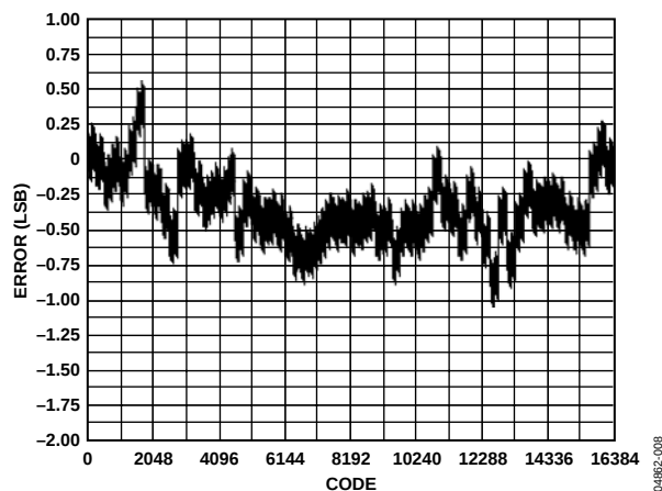
Figure 8. AD9736 INL, 25°C, 10 mA FS
