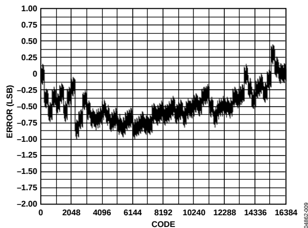
Figure 9. AD9736 INL, 85°C, 10 mA FS
