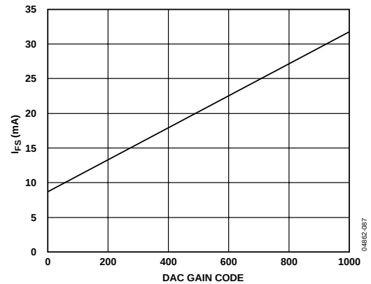
Figure 87. I_{FS} vs. DAC Gain Code
