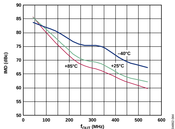
Figure 44. AD9736 IMD vs. f_{OUT} over Temperature, 1.2 GSPS
