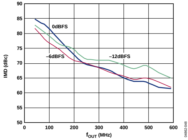
Figure 48. AD9736 IMD vs. f_{OUT} over A_{OUT} , 25°C, 1.2 GSPS
