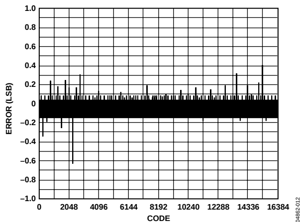
Figure 12. AD9736 DNL, 85°C, 10 mA FS
