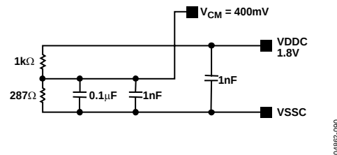
Figure 90. DACCLK V_{CM} Generator Circuit
