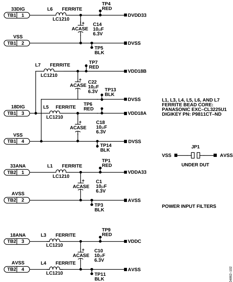
Figure 102. Power Supply Inputs for AD973x Evaluation Board, Rev. F
