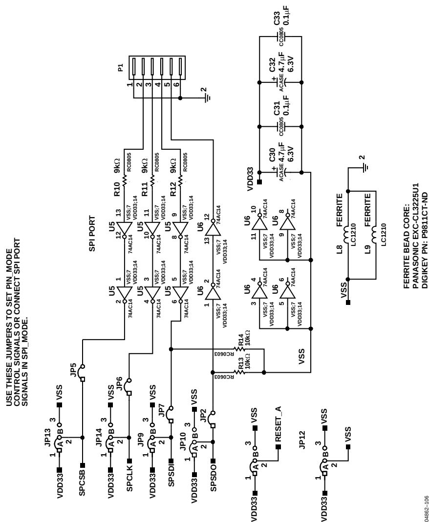
Figure 106. SPI Port Interface, AD973x Evaluation Board, Rev. F
