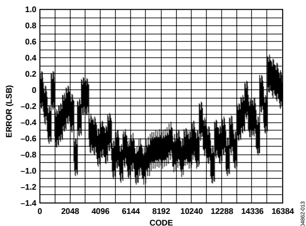
Figure 13. AD9736 INL, -40°C, 20 mA FS
