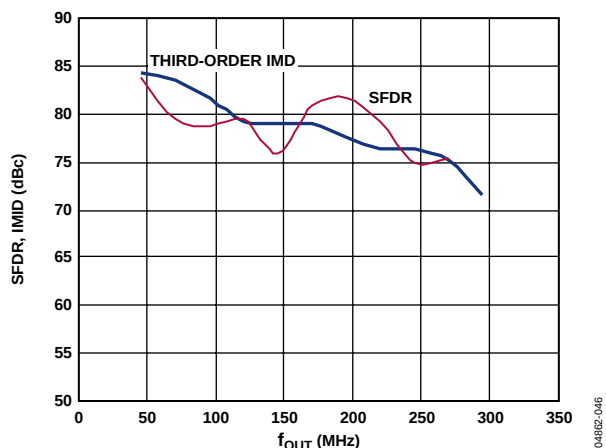
Figure 46. AD9736 IMD and SFDR vs. f_{OUT} , 25°C, 1.2 GSPS, 2x Interpolation
