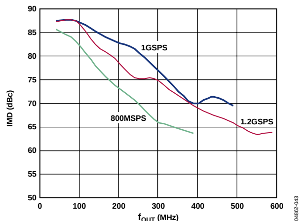
Figure 43. AD9736 IMD vs. f_{OUT} over f_{DAC} at 25°C
