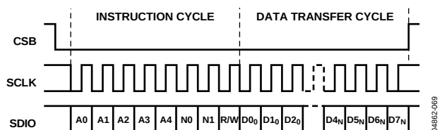
Figure 69. Serial Register Interface Timing, LSB-First Write
