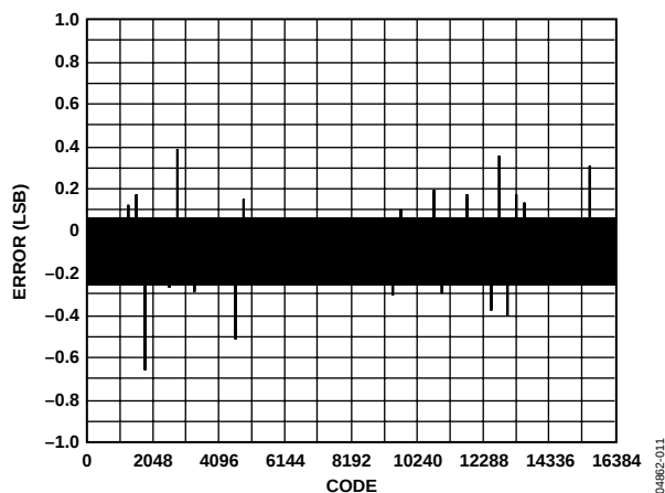
Figure 11. AD9736 DNL, 25°C, 10 mA FS
