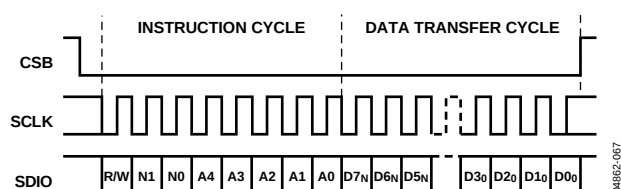
Figure 67. Serial Register Interface Timing, MSB-First Write
