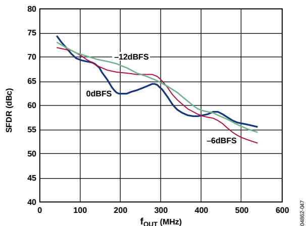
Figure 47. AD9736 SFDR vs. f_{OUT} over A_{OUT} , 25°C, 1.2 GSPS
