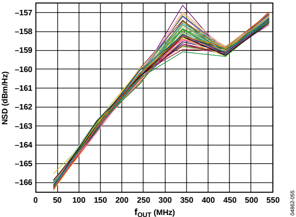
Figure 55. AD9736 1-Tone NSD vs. f_{OUT} over 50 Parts, 1.2 GSPS, 25°C
