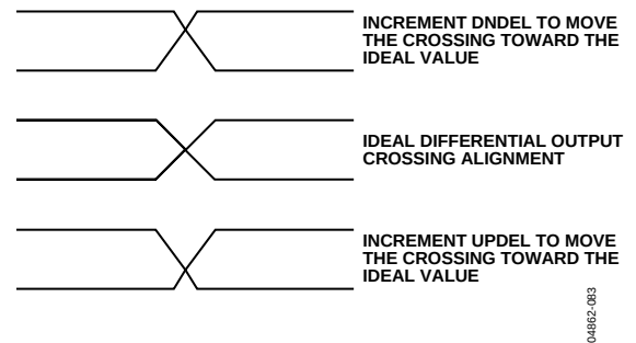
Figure 83. Effect of UPDEL and DNDEL
