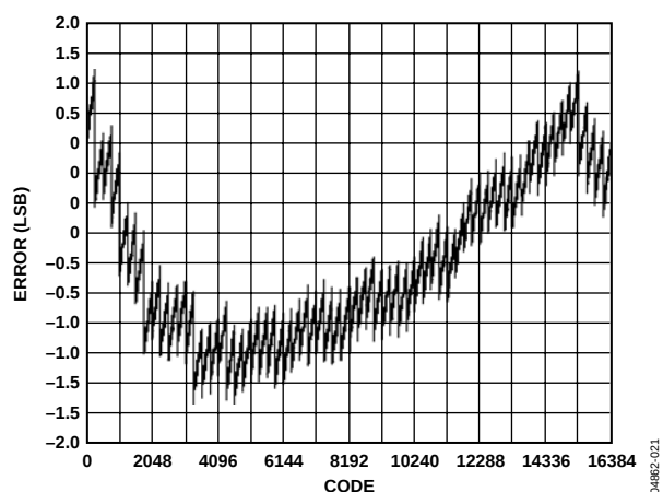
Figure 21. AD9736 INL, 85°C, 30 mA FS
