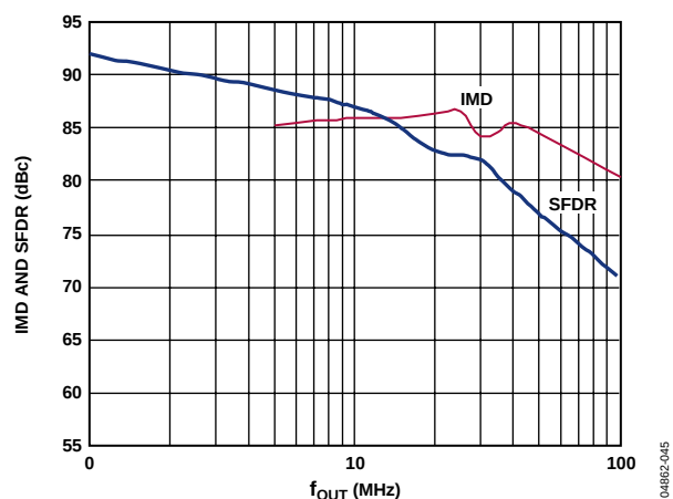
Figure 45. AD9736 Low Frequency IMD and SFDR vs. f_{OUT} , 25°C, 1.2 GSPS
