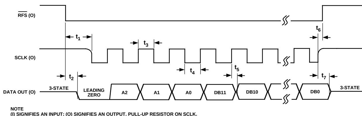
Figure 8. Self-Clocking (Master) Mode Output Register Read
