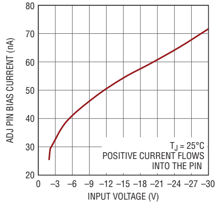
ADJ Pin Bias Current
