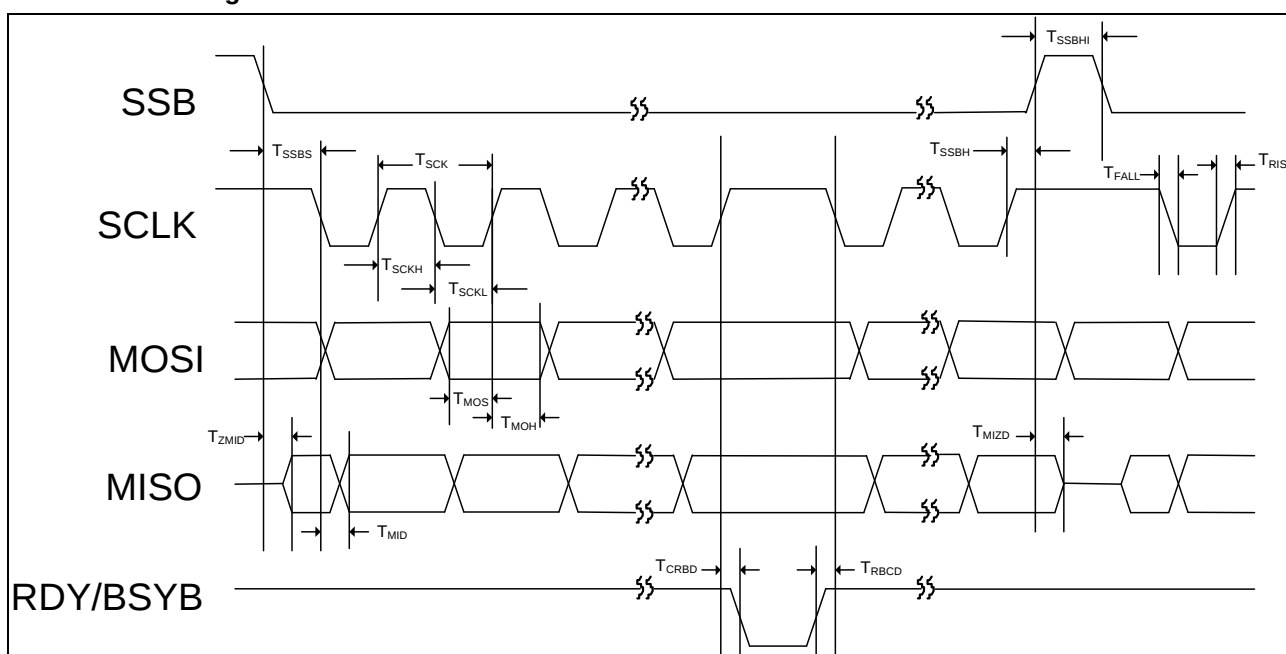
Figure 0-1 SPI Timing
