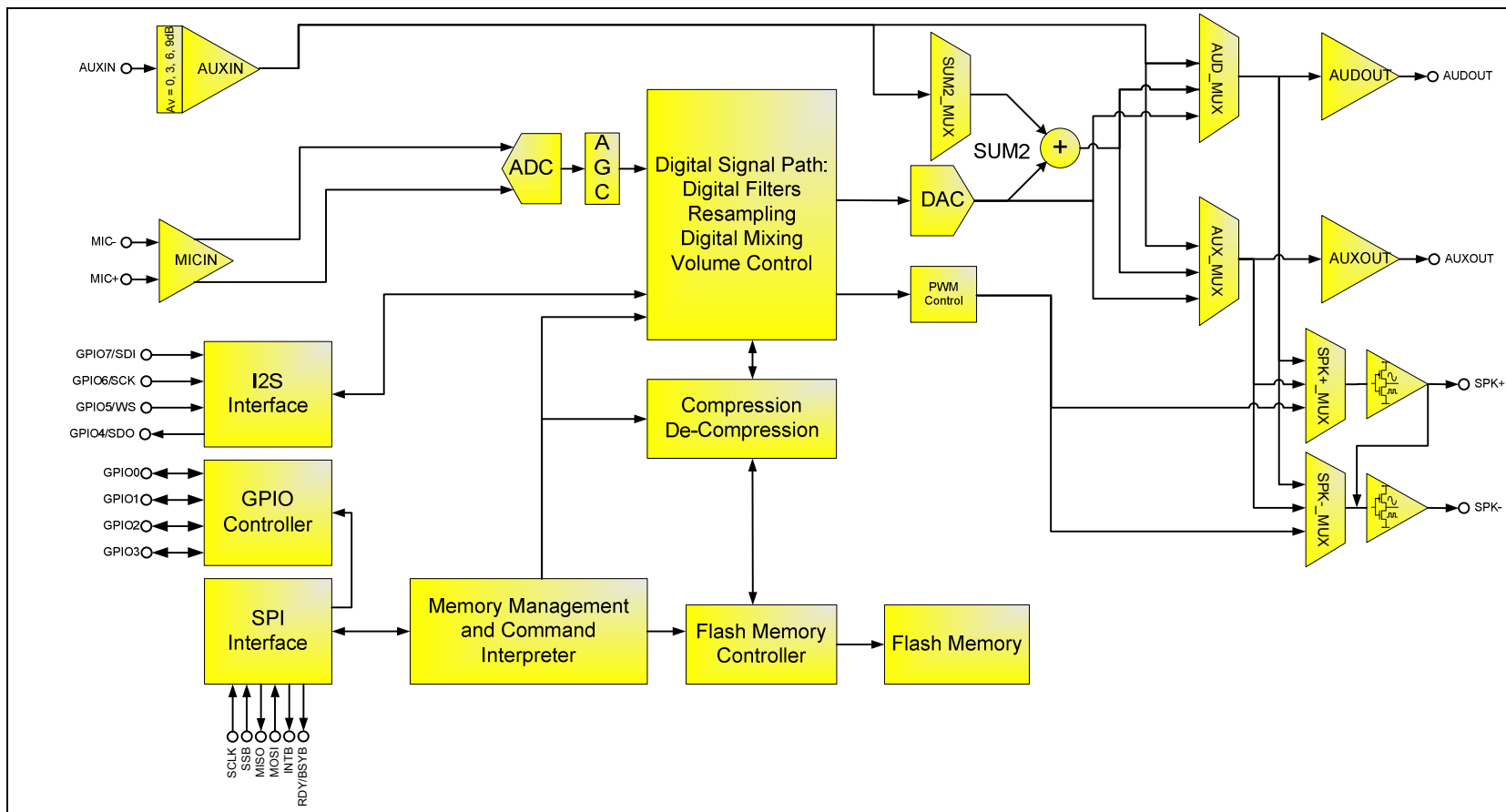
Figure 3-2 ISD15100 Block Diagram, MICIN Selected
