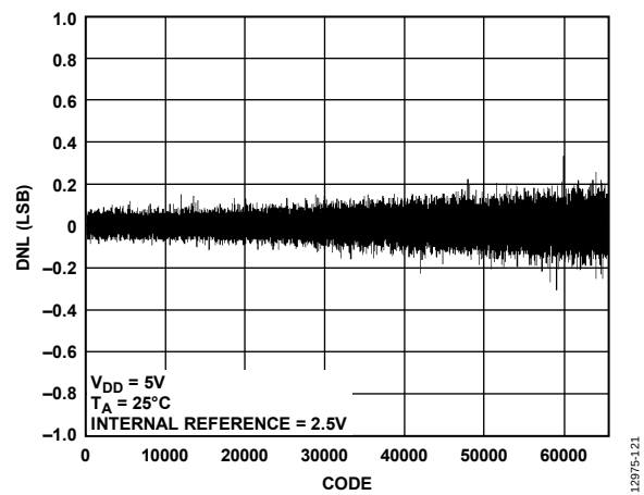
Figure 14. Differential Nonlinearity (DNL) vs. Code
