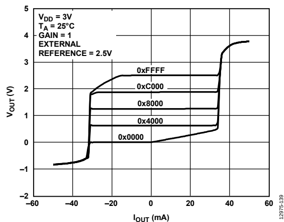
Figure 29. Source and Sink Capability at 3 V
