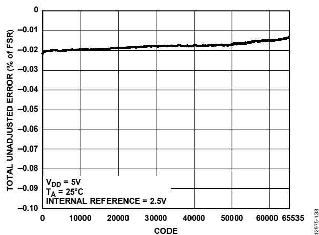
Figure 24. Total Unadjusted Error (TUE) vs. Code
