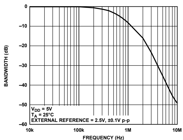
Figure 41. Multiplying Bandwidth, External Reference = 2.5 V, \pm 0.1 V p-p, 10 kHz to 10 MHz
