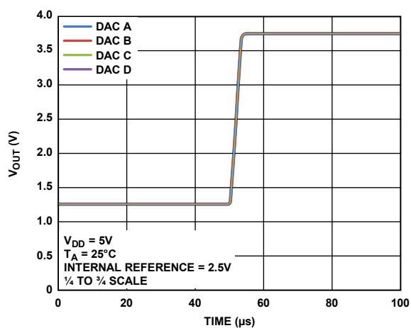
Figure 31. Settling Time
