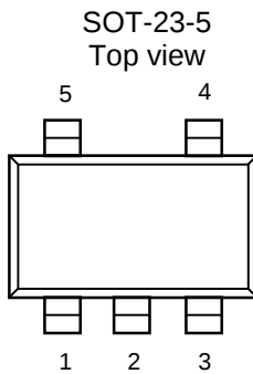
Figure 3 Pin Configuration
