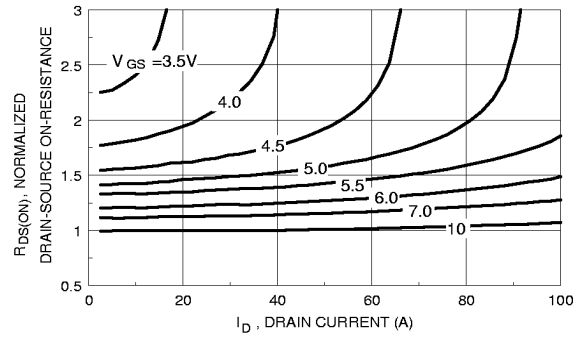
Figure 2. On-Resistance Variation with Drain Current and Gate
