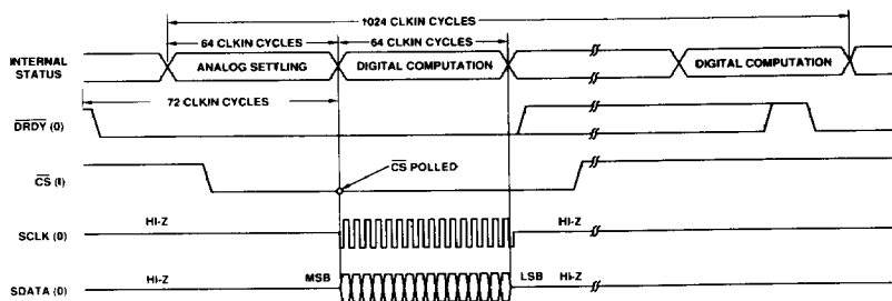
Figure 20. Timing Diagram for SSC Data Transmission Mode
