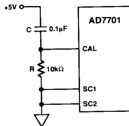
Figure 17. Power-On Reset Circuit
