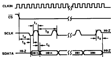
Figure 5. SSC Mode Timing Diagram
