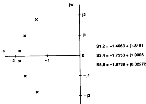
Figure 11. Normalized Pole-Zero Plot of AD7701 Filter
