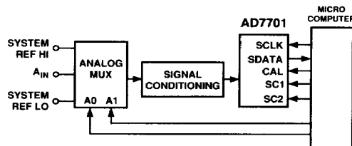
Figure 16. Typical Connections for System Calibration
