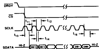
Figure 4b. SEC Mode Timing Diagram
