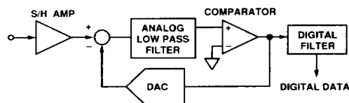
Figure 8. General Sigma Delta ADC
