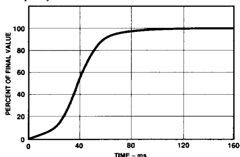
Figure 12. AD7701 Step Response
