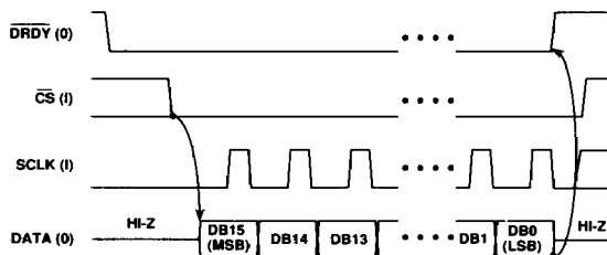
Figure 22. Timing Diagram for the SEC Mode
