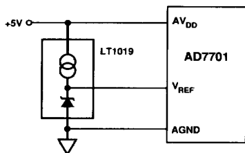
Figure 14. Typical External Reference Connections
