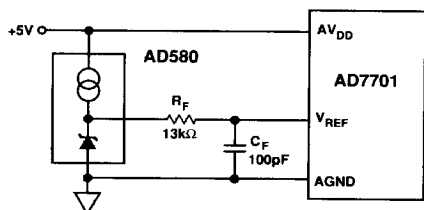
Figure 15. Filtered Reference Input
