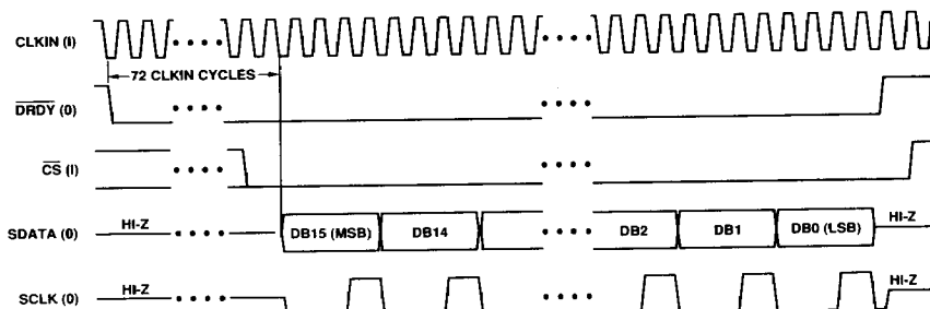
Figure 21. SSC Mode Showing Data Timing Relative to SCLK
