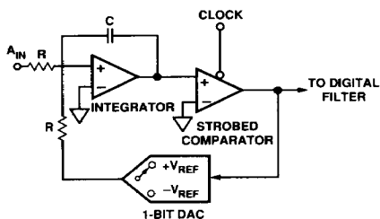
Figure 9. Basic Charge-Balancing ADC
