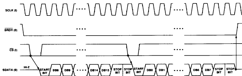
Figure 23. Timing Diagram for Asynchronous Communications Mode
