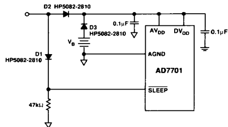
Figure 19. Battery Backup of Calibration Data
