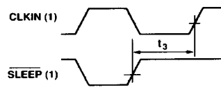
2b. SLEEP Mode Timing
