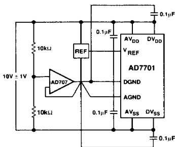
Figure 18. Single Supply Operation
