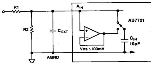
Figure 13. Equivalent Input Circuit and Input Attenuator
