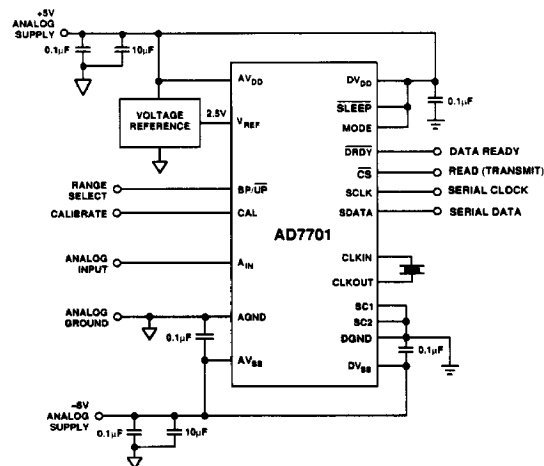
Figure 7. Typical System Connection Diagram
