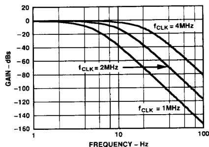
Figure 10. Frequency Response of AD7701 Filter
