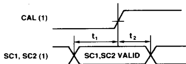
2a. Calibration Control Timing
