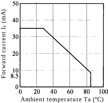
Diode IF-Ta CHARACTERISTICS DIAGRAM
