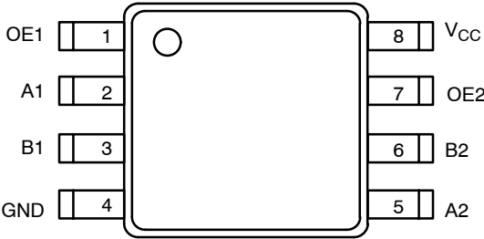
Figure 3. US8/Micro8 (Top View)
