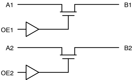
Figure 4. Logic Diagram
