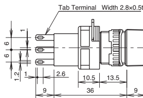
Solder/Tab Terminal
