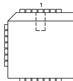
PLCC 28 A SUFFIX CASE 776AA
