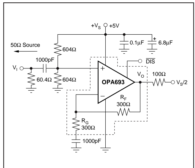
Figure 4. AC-Coupled, G = +2\text{V/V} , Single-Supply Specification and Test Circuit.
