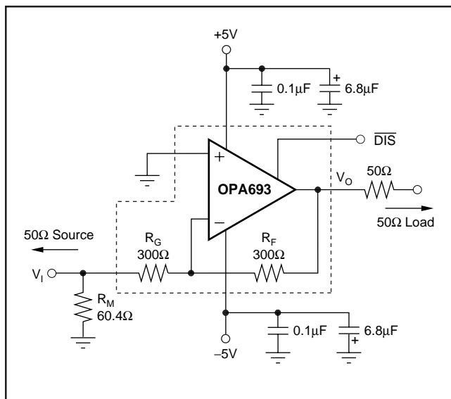
Figure 3. DC-Coupled, G = -1\text{V/V} , Bipolar-Supply Specification and Test Circuit.
