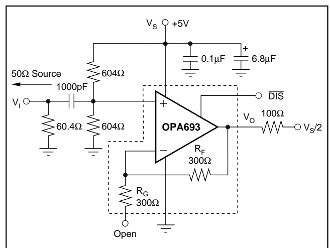
Figure 5. AC-Coupled, G = +1\text{V/V} , Single-Supply Specification and Test Circuit.
