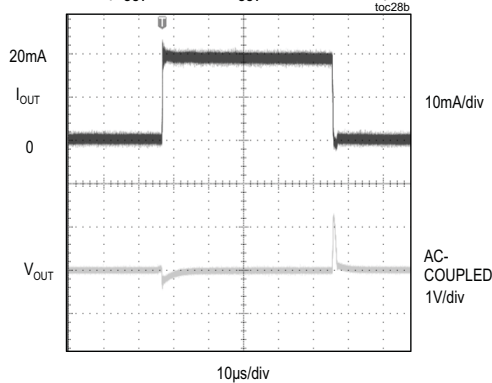
LOAD TRANSIENT ( V_{OUT} = 4.096V , C_{OUT} = 0 , 0 TO 20mA)
