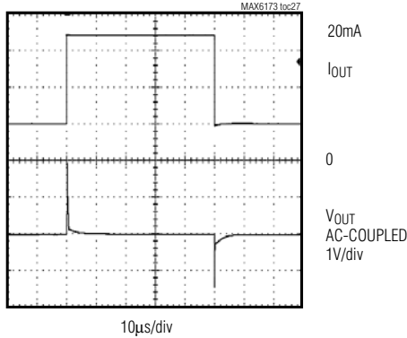
LOAD TRANSIENT ( V_{OUT} = 2.5V , C_{OUT} = 0 , 0 TO 20mA)
