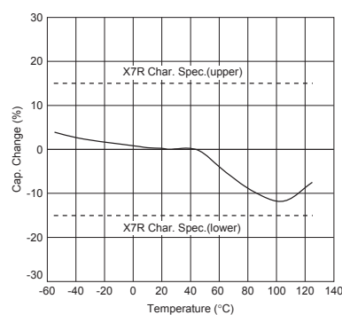
X7R Characteristics
