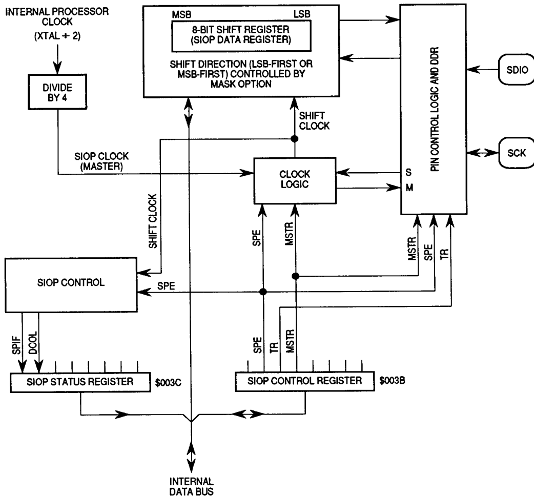
SIOP Block Diagram
