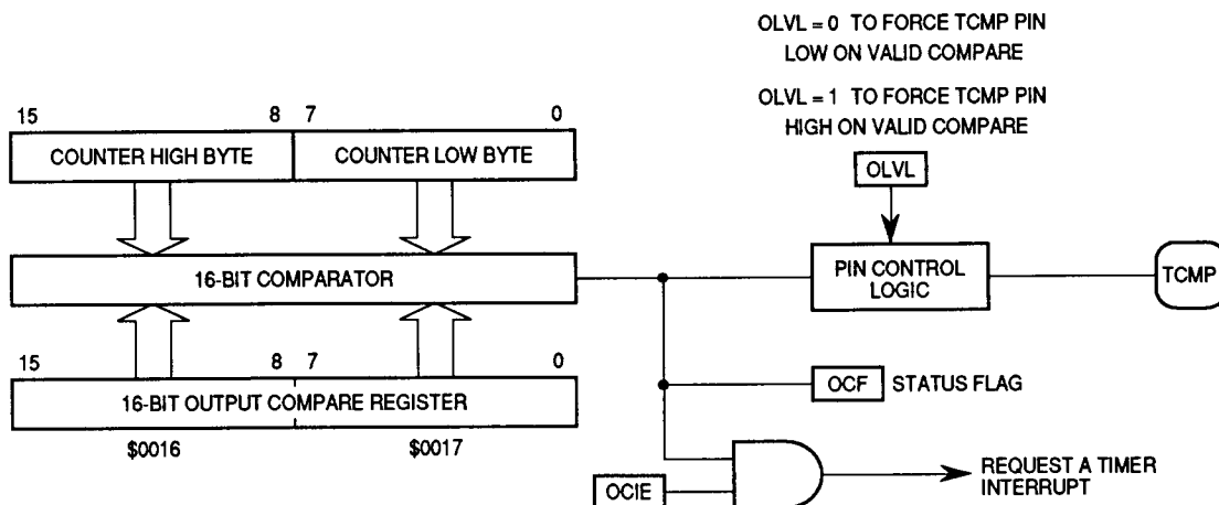
Output Compare Operation
