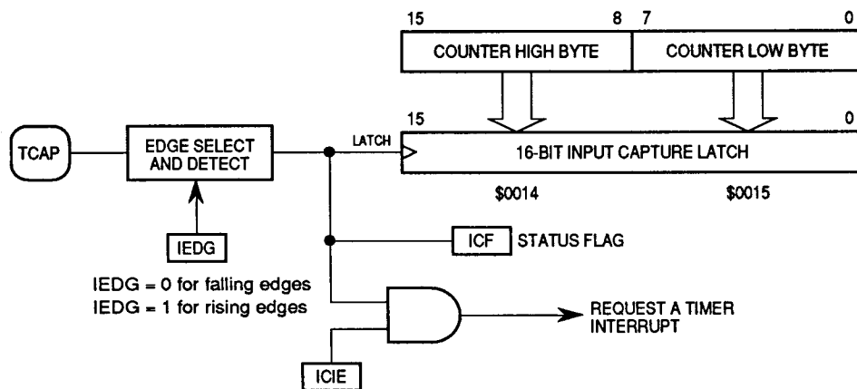
Input Capture Operation
