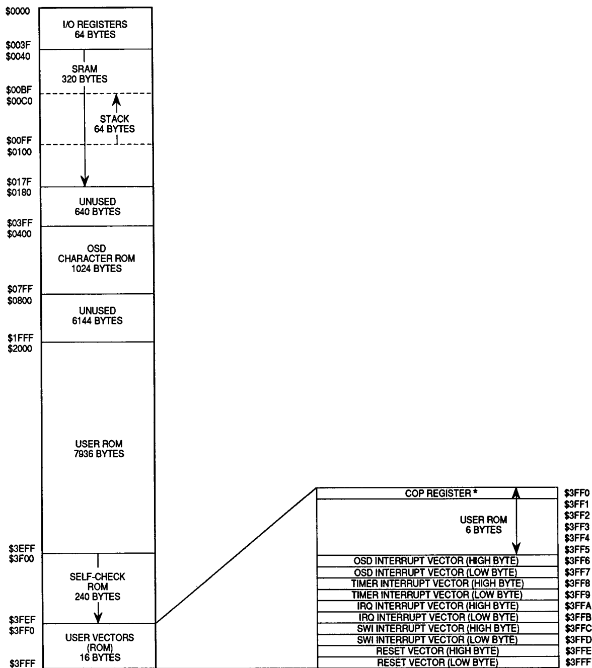
Memory Map (Continued)
