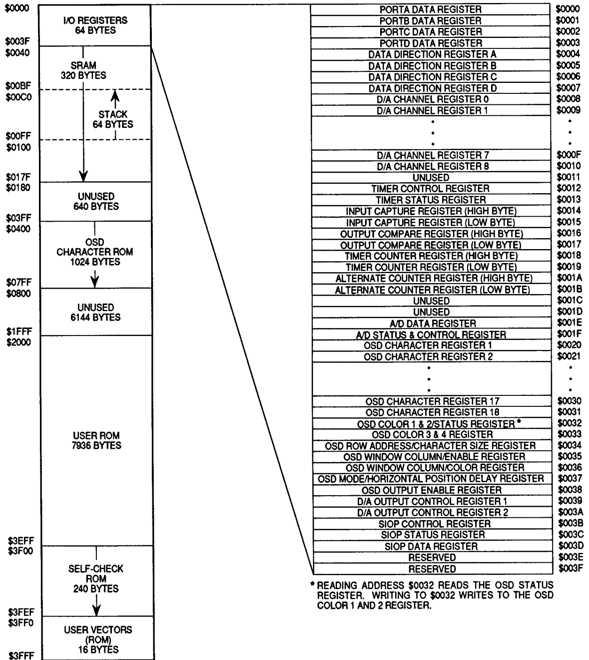
Memory Map
