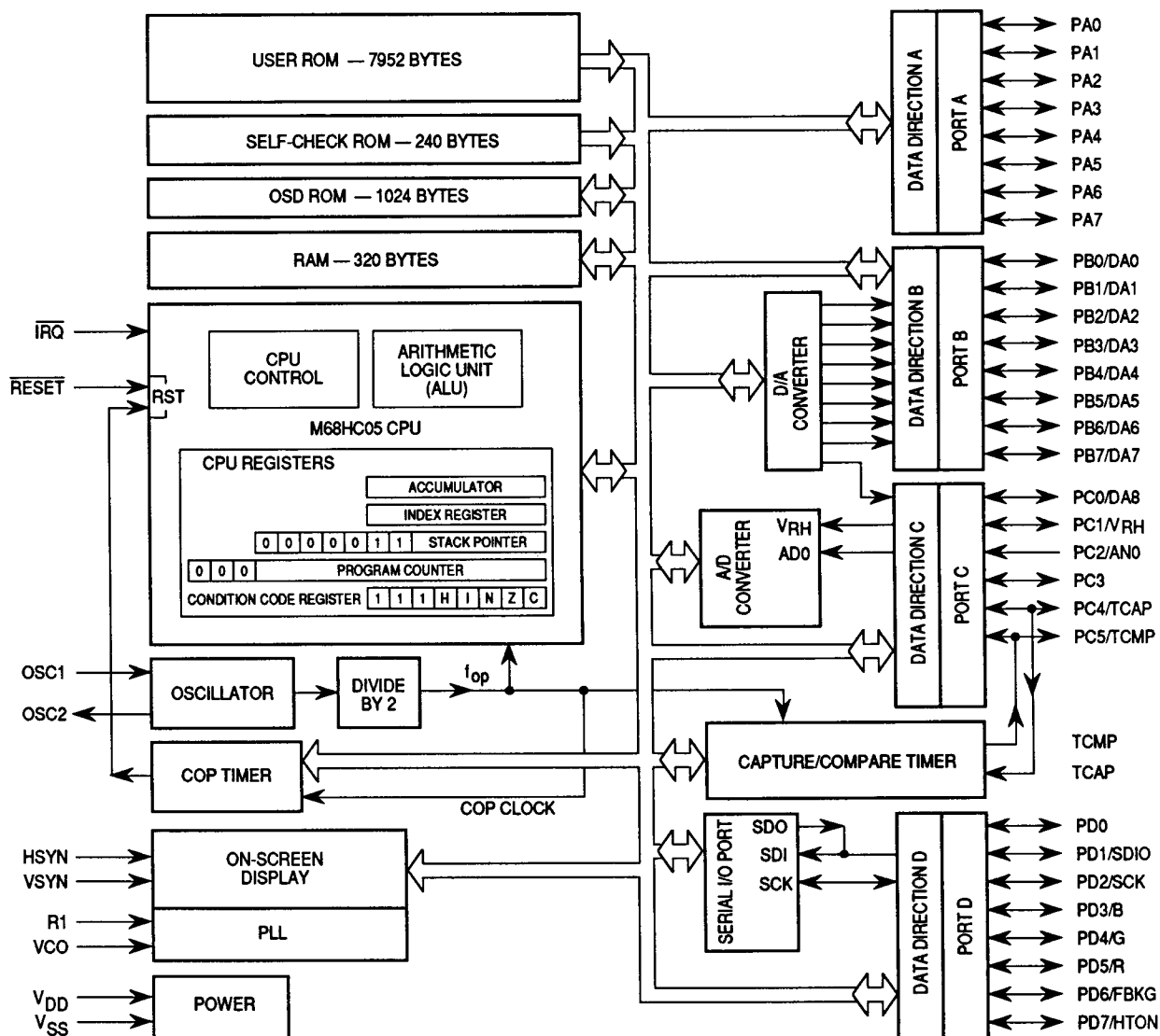
MCU Block Diagram
