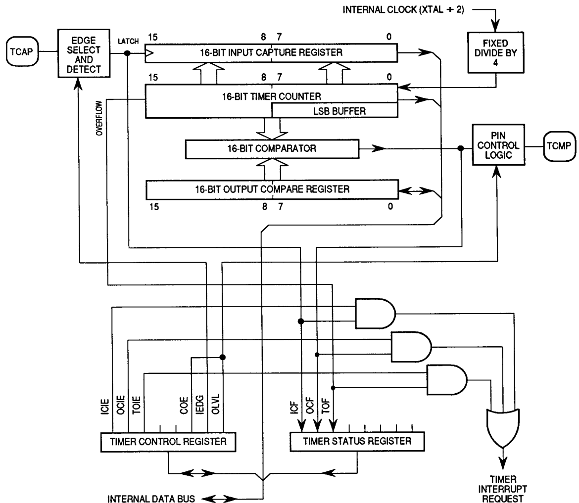
Capture/Compare Timer Block Diagram
