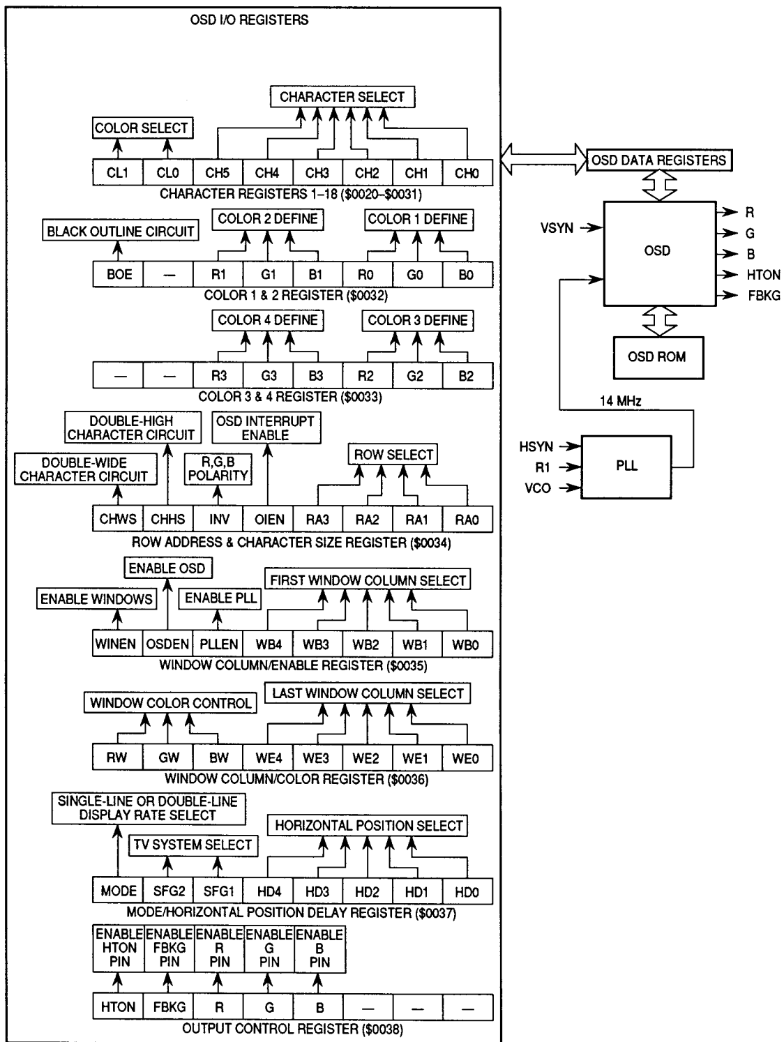
OSD Block Diagram
