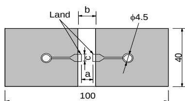
Fig.1 (in mm)
