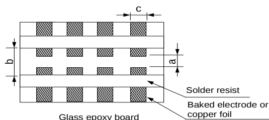
Fig.3 (in mm)
