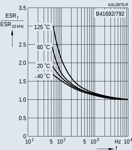
Frequency characteristics of ESR at different temperatures Typical behavior
