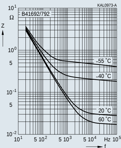
Impedance Z versus frequency f at different temperatures Typical behavior for 2200 \mu F/25 V
