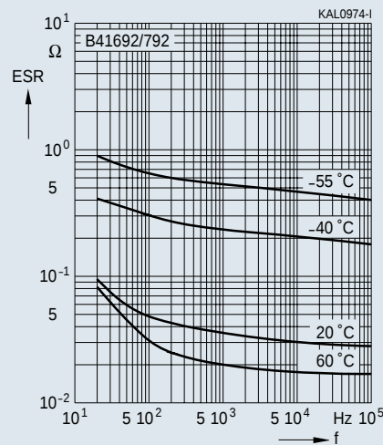
Equivalent series resistance ESR versus frequency f at different temperatures Typical behavior for 2200 \mu F/25 V
