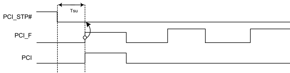
Figure 3. PCISTOP# Assertion Waveform
