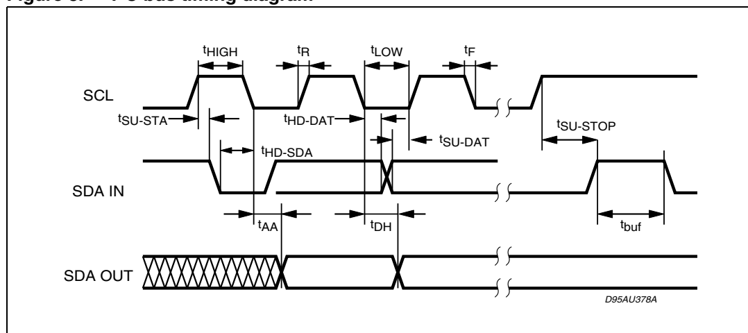
Figure 8. I 2 C bus timing diagram
