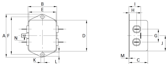
Connection style -06, 1 A types
