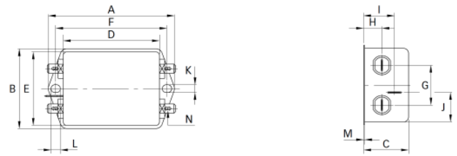
Connection style -06, 3 to 20 A types
