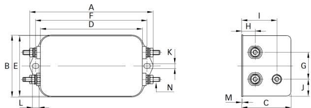
Connection style -08, 20 and 30 A types
