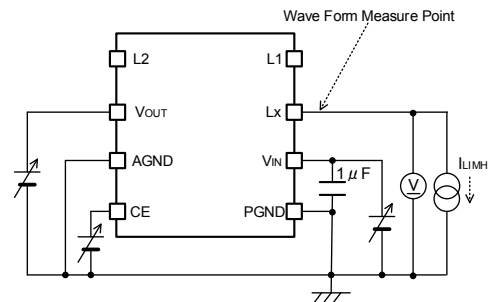
< Circuit No.⑥ >
