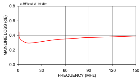
ZDC-20-3-75 MAINLINE LOSS
