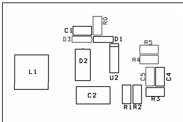
(COMPONENT - TOP)
