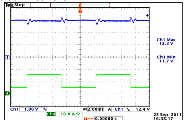
12V OUT, 230VAC, 25% TO 75% LOAD STEP
